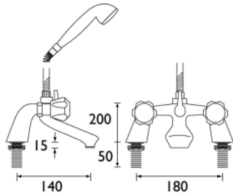
1500mm HOSE, HANDSET & WALL BRACKET
