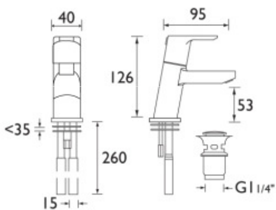
Small Basin Mixer
